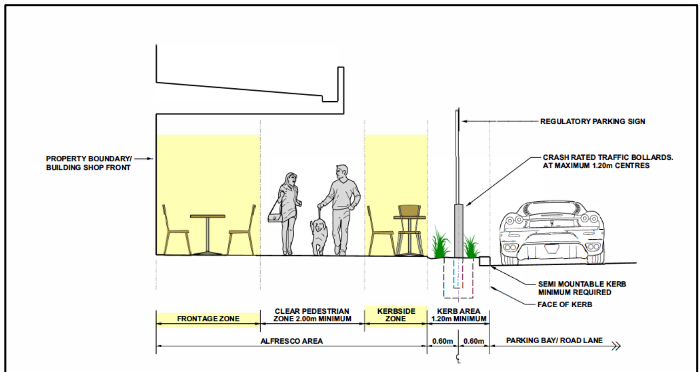
Figure 1- Sectional Elevation View Outdoor Eating Facility
