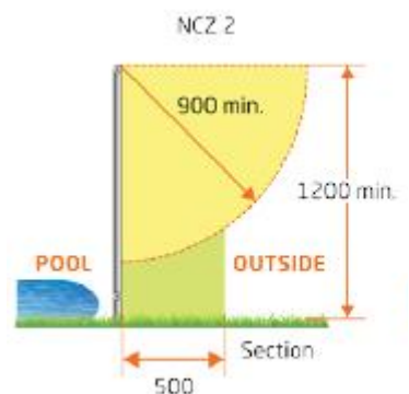
900mm non-climbable zone from top of barrier outside Nothing within 500mm of the outside of the barrier
