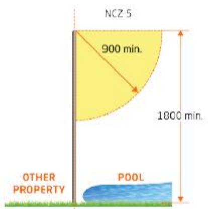
boundary fence forming part of the barrier
