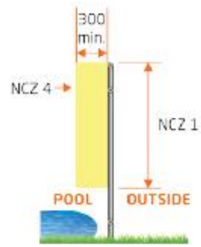
300mm non-climbable zone inside barrier
