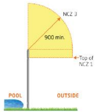
900mm non-climbable zone from top of barrier above
